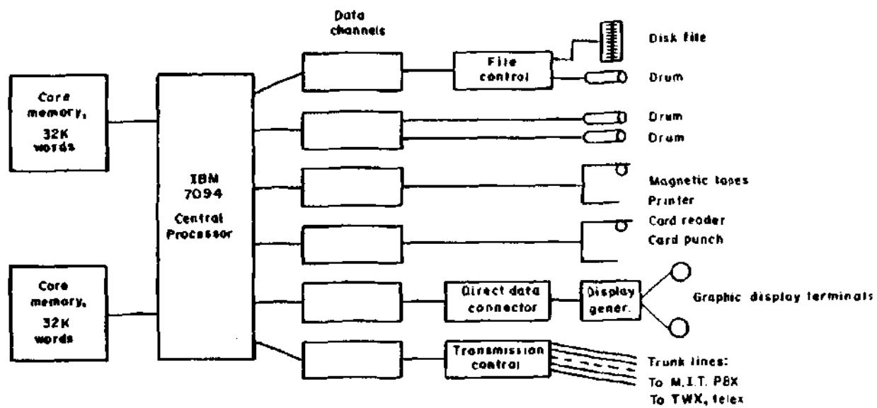
FIG. 1. Structure of MAC computer installation at the end of 1965.
