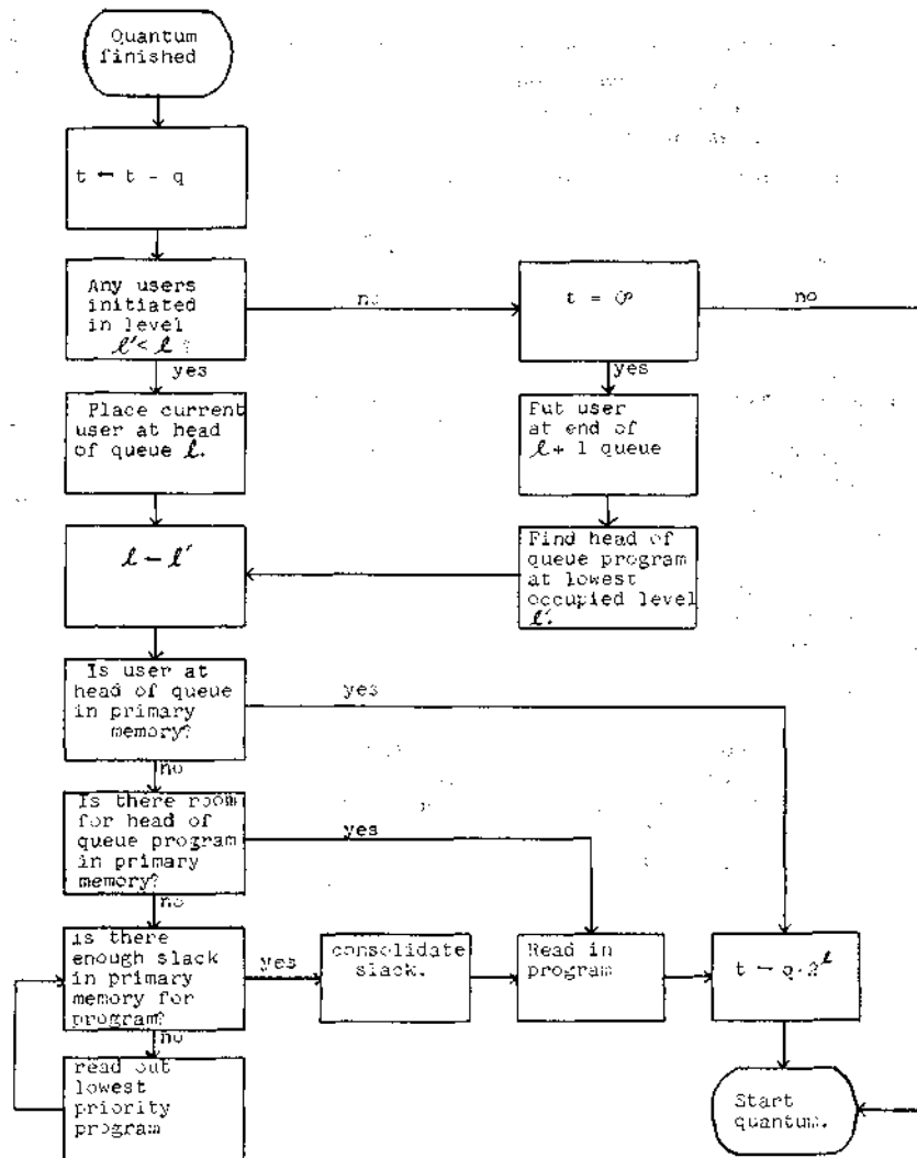
Figure 2. Flow Chart of Multi-Level Scheduling Algorithm
