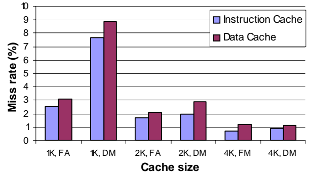
Figure 12: Cache miss rate for different sizes of caches with direct mapped and fully associative organization.
