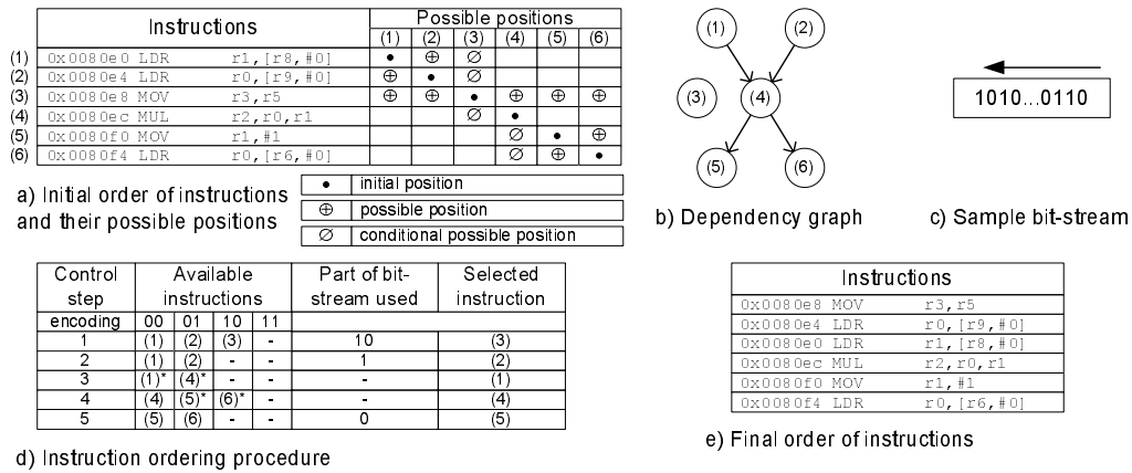
Figure 4: An example of constraint embedding for the instruction rescheduling transform.
